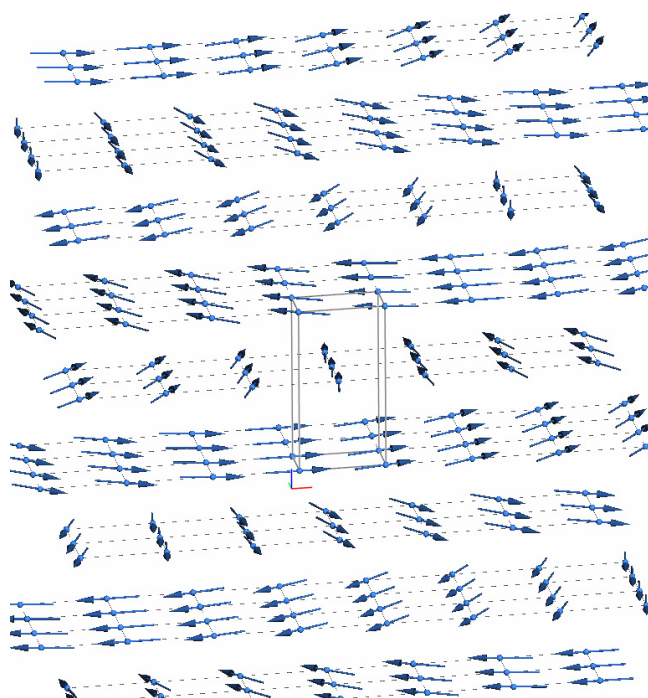
Figure 4. Magnetic structure of \text{Cr}_{0.5}\text{TiSe}_2 . The l = (000) crystallographic cell is indicated. (This figure is in colour only in the electronic version)
